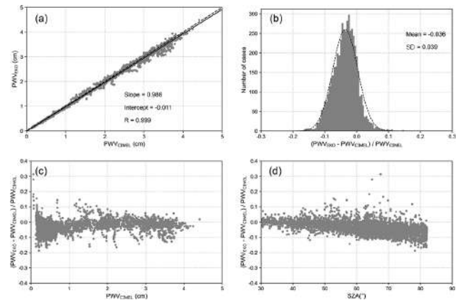
Figure 10. PWV retrievals from EKO using the spectral approach in the 880–1000 nm region compared to the synchronous data of CE-318 in the measuring period (a), histogram of relative difference among \text{PWV}_{\text{EKO}} and \text{PWV}_{\text{CIMEL}} (b), and the relative difference plotted against \text{PWV}_{\text{CIMEL}} (c) and solar zenith angle (d).
