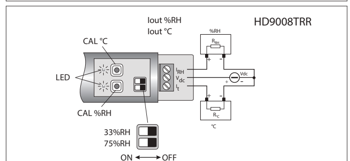
Fig. 3 - Connection and programming of HD9008TRR
